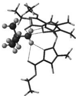
Figure 1. The structure of [(\text{CH}_3)_3\text{CNH}_3][\text{Tp}^{\text{CO}_2\text{EtMe}}] ( 1 ). The host \text{Tp}^{\text{CO}_2\text{EtMe}} is depicted as a tube model while the guest (\text{CH}_3)_3\text{CNH}_3 is shown as a ball-and-stick structure. Dotted lines indicate the bifurcated hydrogen bonds.
